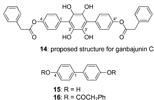
Figure 1. Structures of ganbajunin C and biphenyls.
